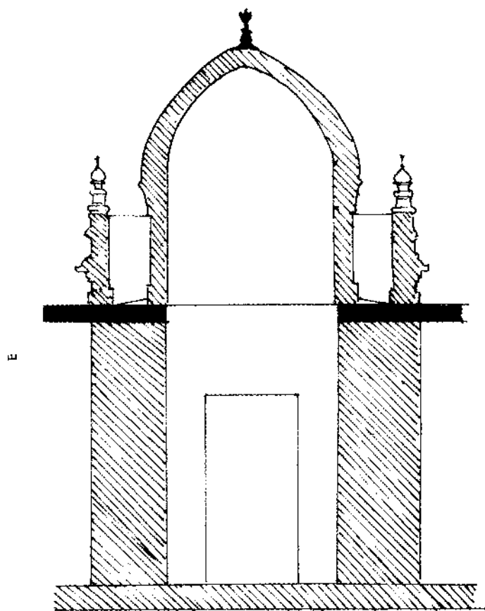
Fig. 102. NatharWali Dargah - Cut Section
